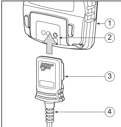
Figure 3. Connecting the IR Link
