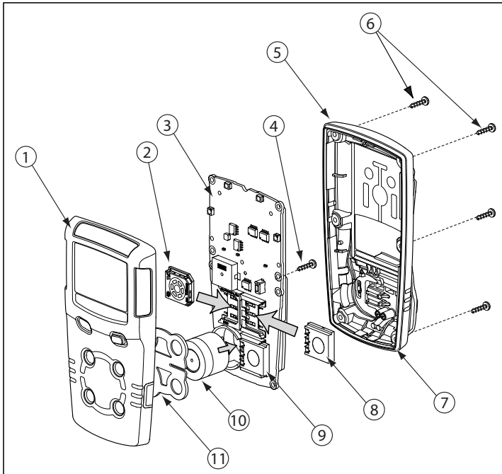
Figure 11. Replacing a Sensor or Sensor Filter
