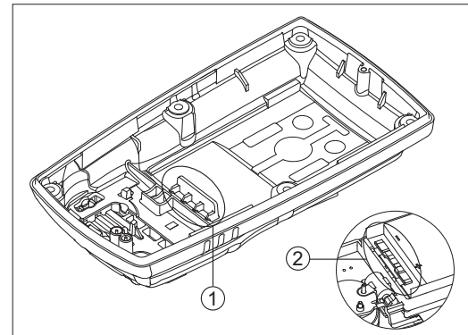
Figure 13. Replacing the Rear Shell
