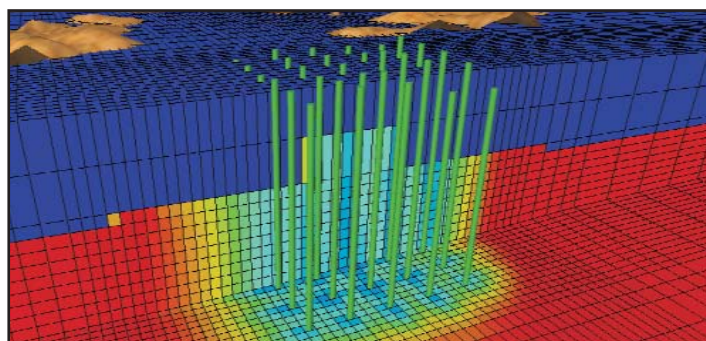
Simulation of ASR using ECLIPSE
