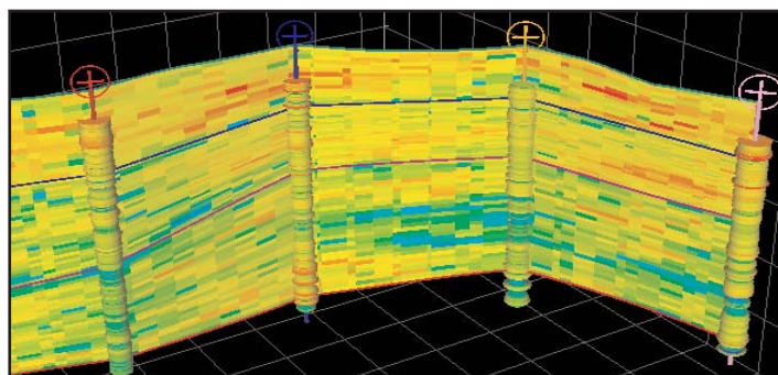
Advanced aquifer modeling using Petrel
